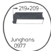
Br 219/160 x 209/120 Talon Konkav
